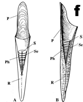
A: Frontal Section B: Lateral Section Ph: Phragmocone P: Proostracum R: Rostrum S: Siphuncle Se: Septum
